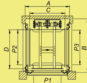
TRIPLE EMBARQUE
