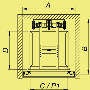
EMBARQUE FRONTAL
